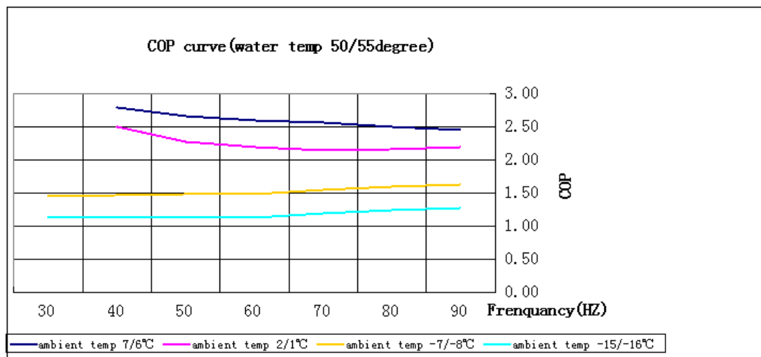
The COP curve of Inverter heat pump H15 at 50/55°C
